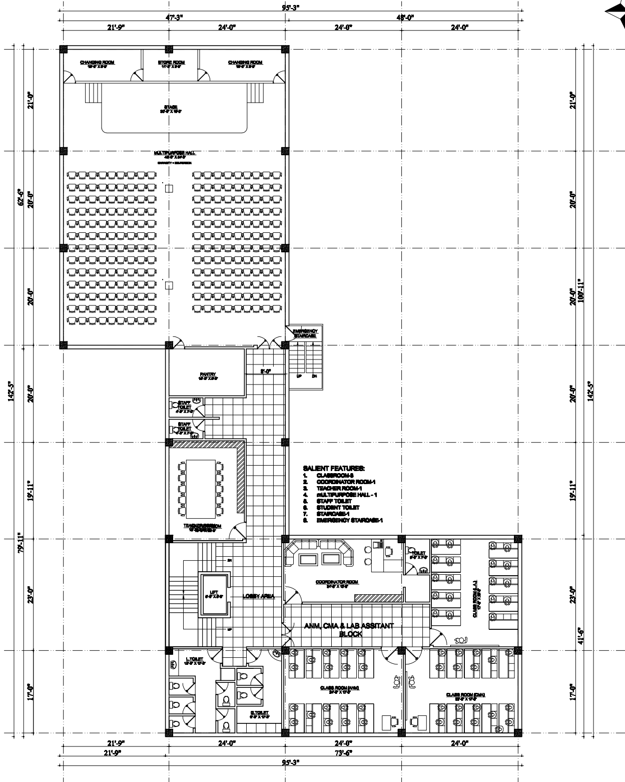
THIRD FLOOR PLAN FLOOR AREA= 6977.65 SQ.FT
